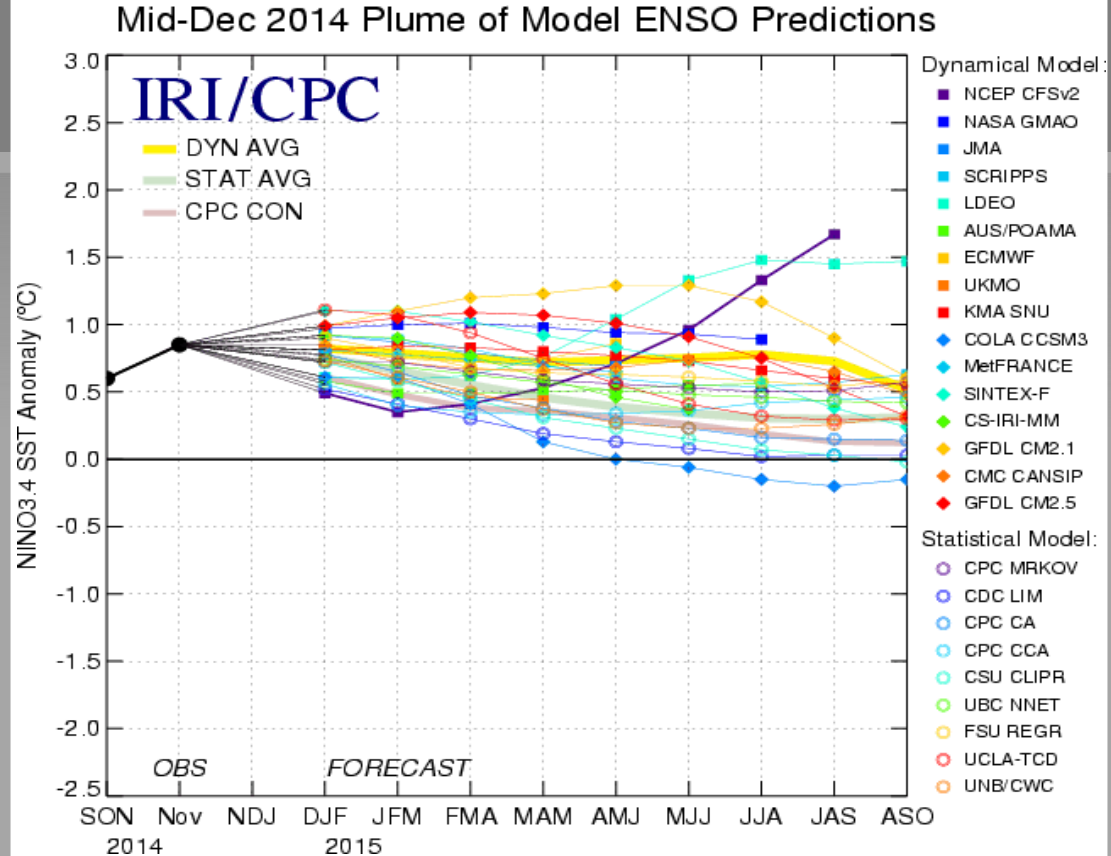
Figure provided by the International Research Institute (IRI) for Climate and Society (updated 16 December 2014).
